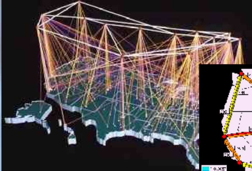
Internet Backbone - 1997
