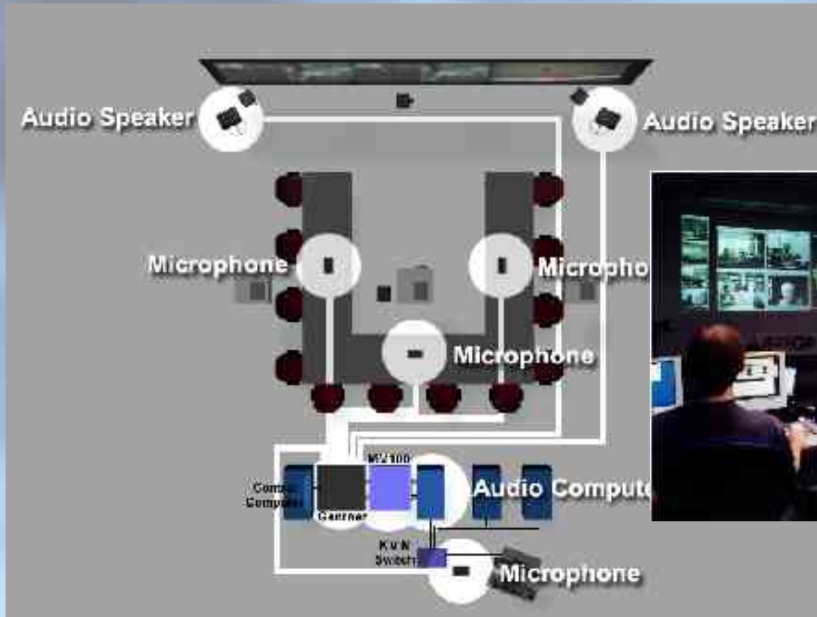
Room-Based Access Grid Node
